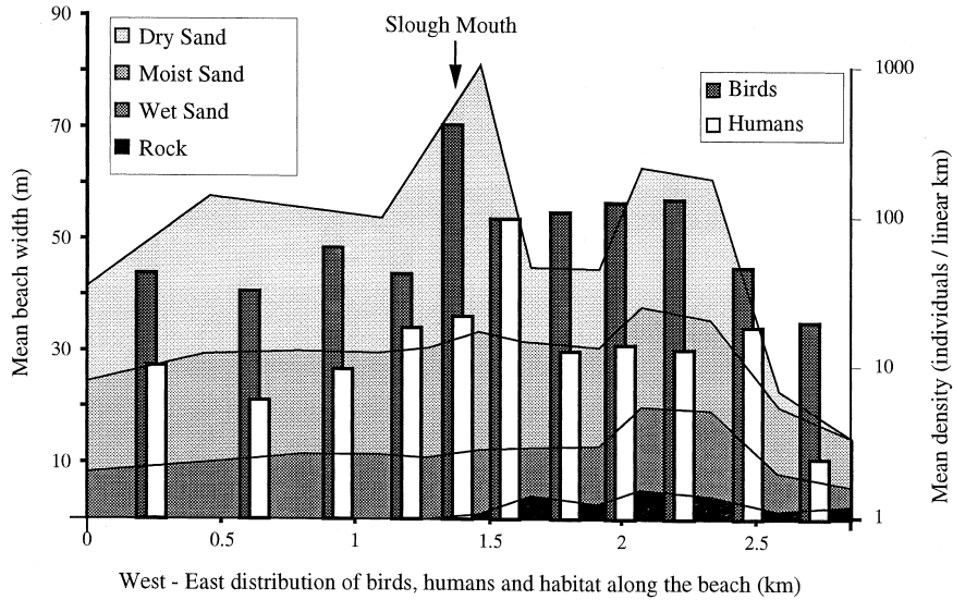
Figure 3. Beach width, substrate type and density of birds and humans along the transect.
