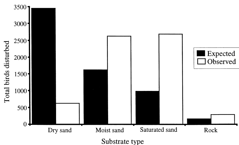
Figure 7. Location of disturbances among substrate type (observed) relative to available substrate type (expected). Expected values for each substrate type are the total number of disturbed birds times the proportion of a particular substrate type recorded for the beach (averaged over all dates). People and birds were generally lower on the beach (moist and saturated), with the exception of a sunbathing area, where most of the people were on the dry sand. The departure from expected, therefore, is most likely because people and birds did not use the habitat evenly (because we did not record habitat use, I could not evaluate this quantitatively).
